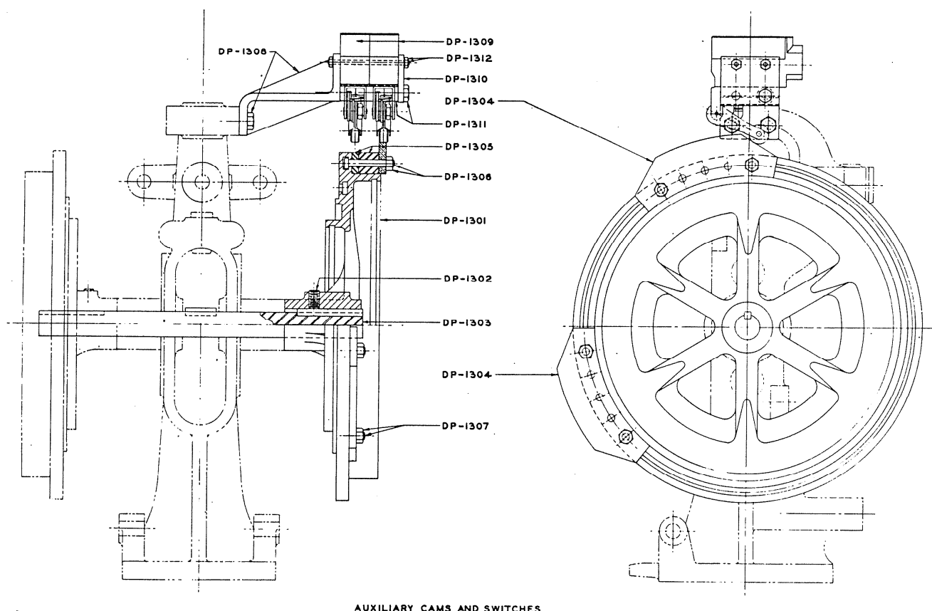
AUXILIARY CAMS AND SWITCHES
