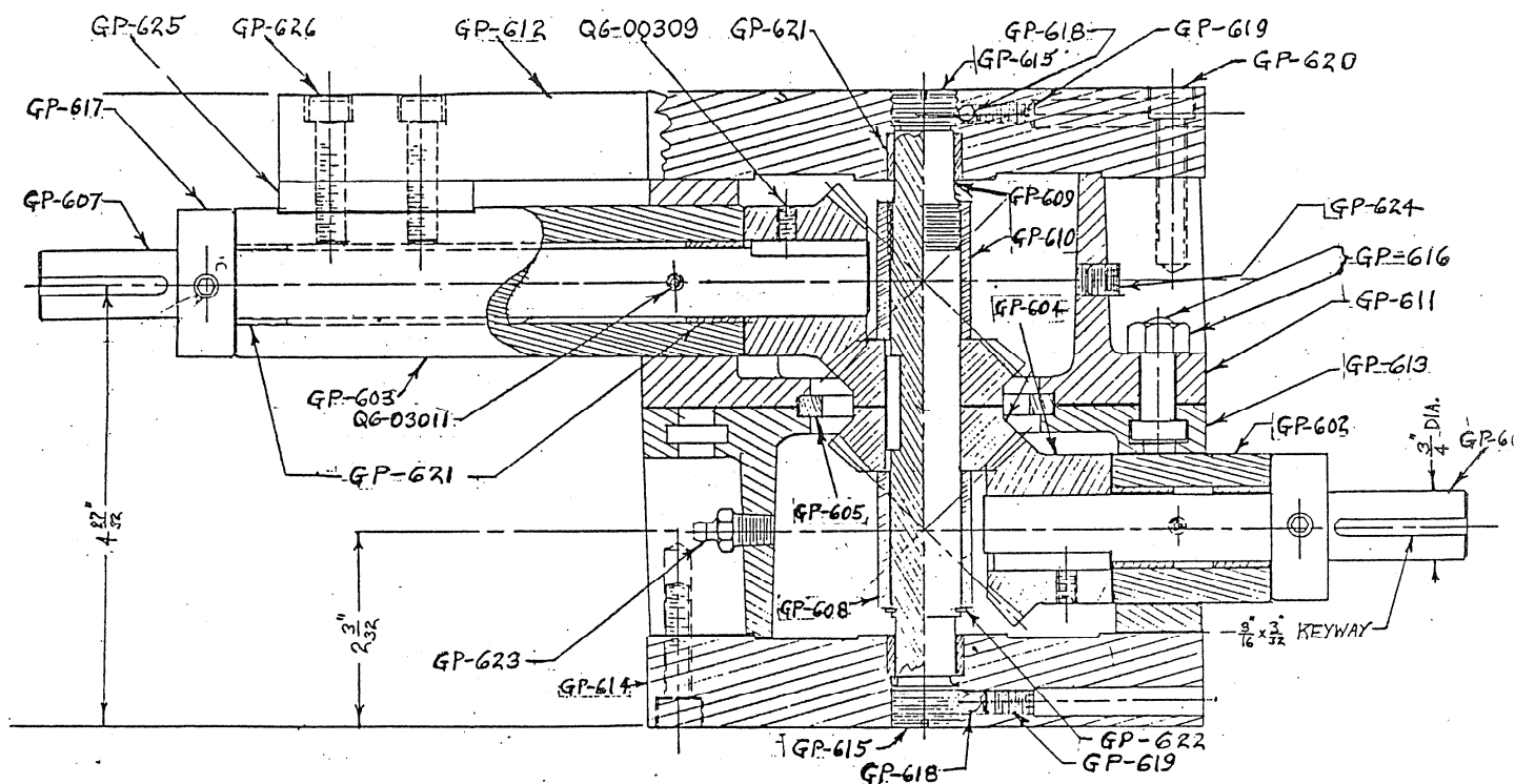
M-815 DIRECTIONABLE BASE (FOR MODEL "D")
