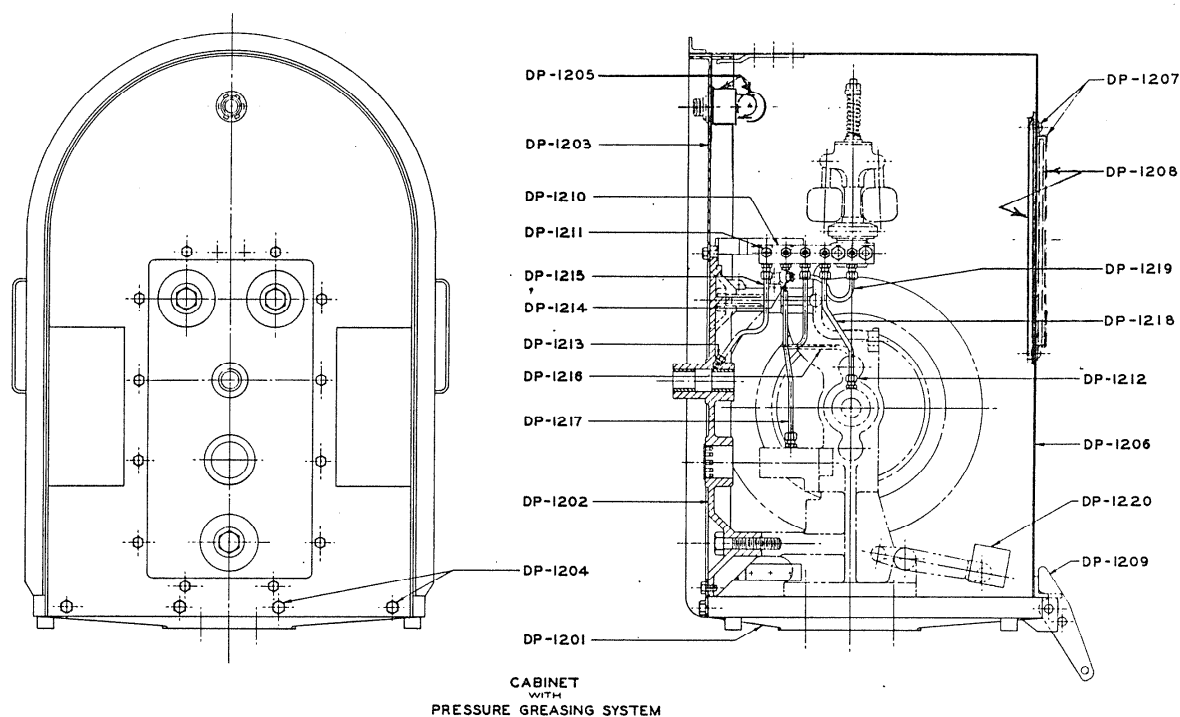
Fig. 12 Drg. DP-D-2055
