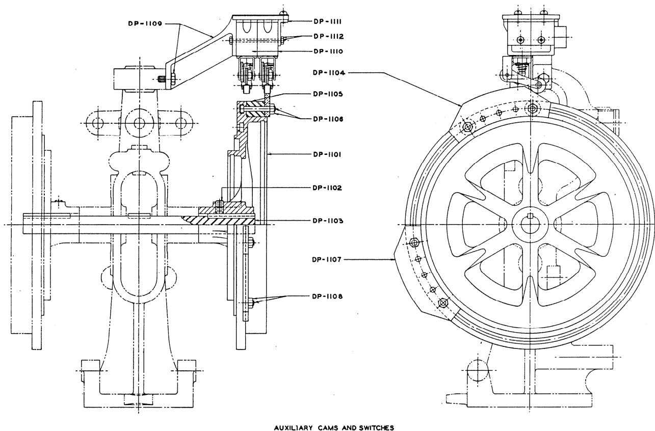
AUXILIARY CAMS AND SWITCHES
